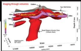
3D resistivity models
