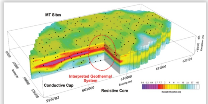
Site deployment and resulting 3D Resistivity model (shown from surface to 3500m).
